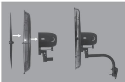
1. Fan motor ,back guard ,and blade assembly.
